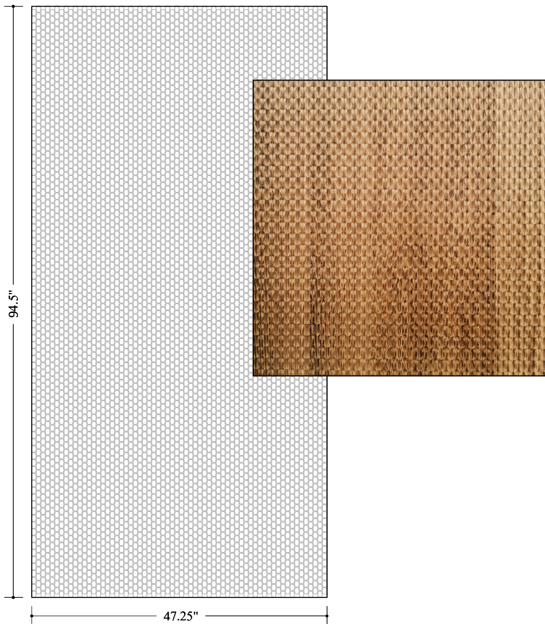
WPFSN209 (scale: 3/4" = 1'-0")
